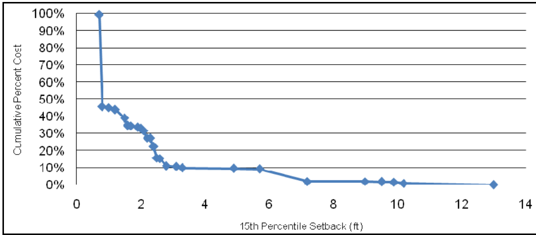
Figure 5-117. Cumulative cost 15th percentile setback in segment analysis with over 6,000 ADT
